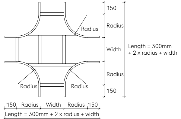
Crossover
