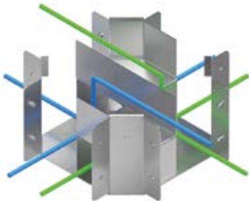
2-compartment
