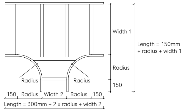
Unequal tee
