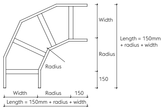
90° flat bend
