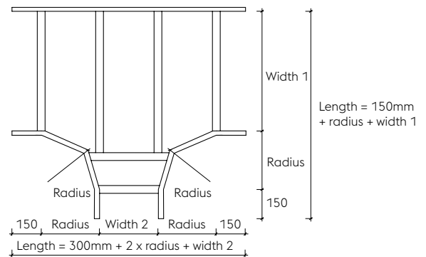
Unequal tee
